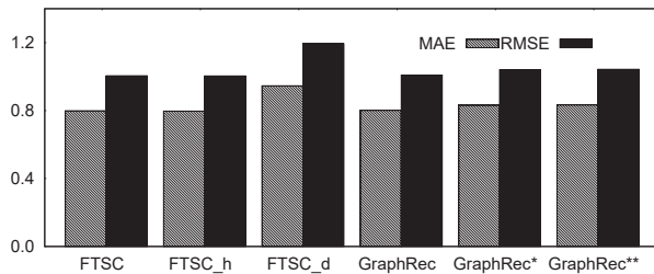
Figure 1: MAE & RMSE for User Recommendation in ML-100k Dataset
