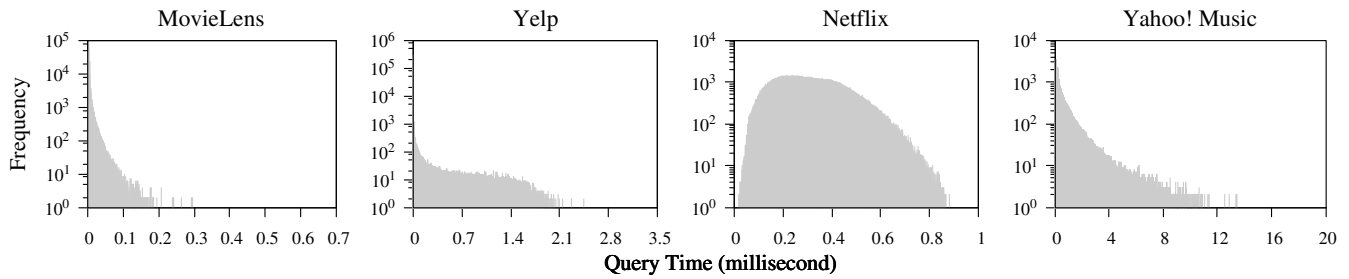
Figure 9: Distribution of Individual Query Costs (F-SIR, k = 1 )
