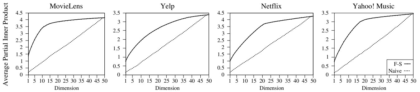
Figure 15: Partial Inner Product Before and After SVD Transformation
