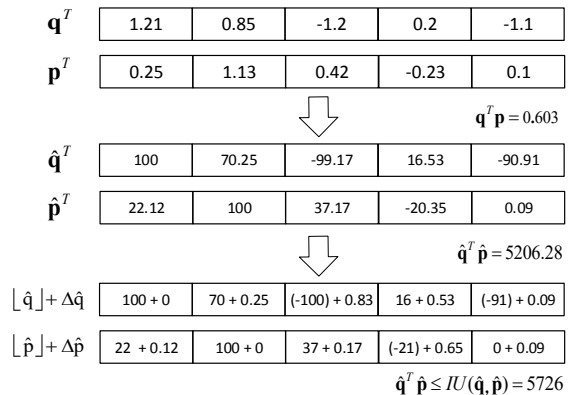
Figure 5: Integer Upper Bound After Scaling
