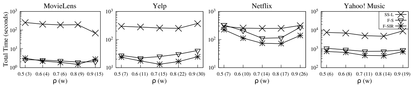
Figure 10: Total Retrieval Times for All Queries for Different \rho(w) Values ( k = 1 )
